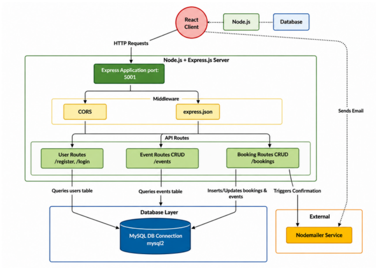
Figure 3.1: Backend Architecture
